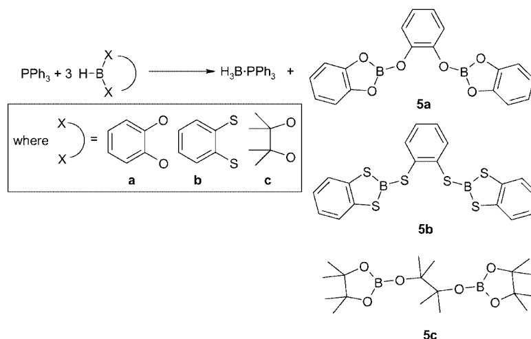
Scheme 3. Formation of disproportionation products 5a , [26a] 5b and 5c [26b] catalyzed by \text{PPh}_3 .
