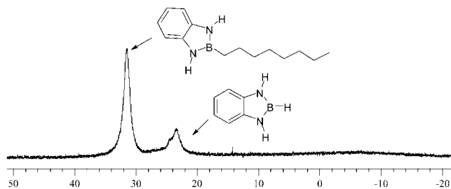
Figure 6. ^{11}\text{B} NMR spectrum (measured in ppm) obtained from the catalyzed hydroboration of 1-octene with 1,3,2-benzodiazaborolane after 24 h at 25 °C.
