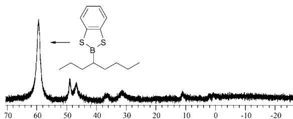
Figure 5. ^{11}\text{B} NMR spectrum (measured in ppm) obtained from the catalyzed hydroboration of trans -4-octene with 1,3,2-benzodithiaborolane.
