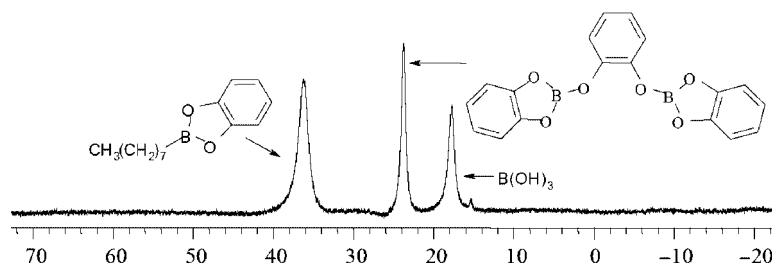
Figure 3. Typical ^{11}\text{B} NMR spectrum of the product mixture of the catalyzed hydroboration of 1-octene with CatBH, which shows a varying distribution of products formed during catalysis.
