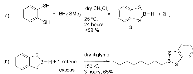
Scheme 2. (a) Synthesis of 1,3,2-benzodithiaborolane ( 3 ). (b) Uncatalyzed hydroboration of 1-octene with 3 . Yields are based on ^{11}\text{B} NMR spectroscopy.
