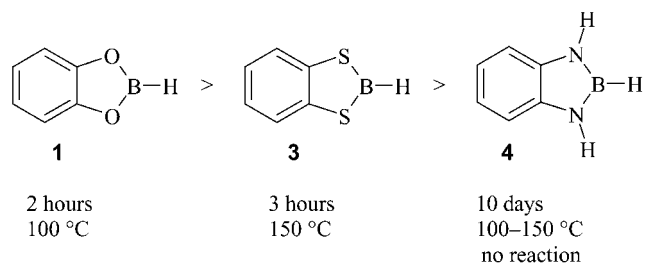
Figure 2. Observed reactivity trend from hydroboration of 1 and 4-octene.
