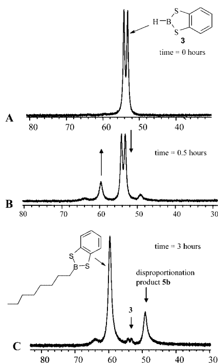
Figure 1. (A) ^{11}\text{B} NMR spectrum of freshly synthesized 1,3,2-benzodithiaborolane in \text{CH}_2\text{Cl}_2 . (B) ^{11}\text{B} NMR spectrum that shows the formation of 2-octyl-1,3,2-benzodithiaboronate ester after 0.5 h and (C) shows the product formation (65%, 21% of 5b and 4% of 3 ) after 3 h.
