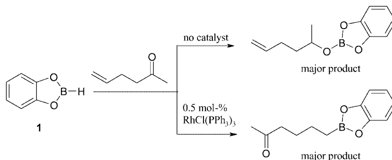
Scheme 1. Uncatalyzed and catalyzed hydroboration of 5-hexen-2-one with catecholborane – altered chemoselectivity.
