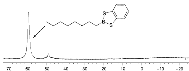
Figure 4. ^{11}\text{B} NMR spectrum (measured in ppm) obtained from the catalyzed hydroboration of 1-octene with 1,3,2-benzodithiaborolane.
